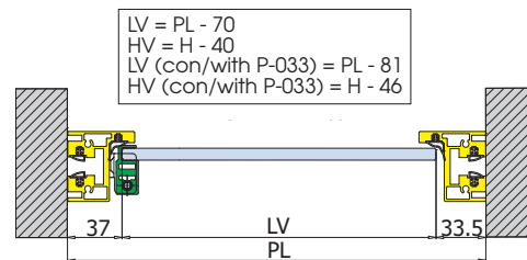
Hinge profile - glass to be glued - on frame TP-250
