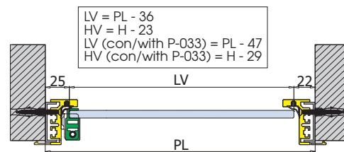
Hinge profile - glass to be glued - on frame TP-100
