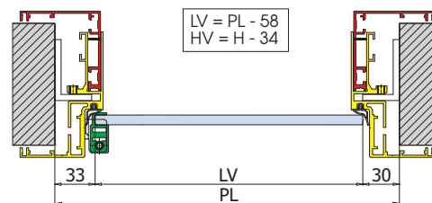
Hinge profile - glass to be glued - on frame TP-250
