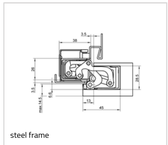
casing frame
