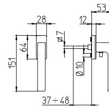
1682/DK-SIC martellina dk drehkipp system
