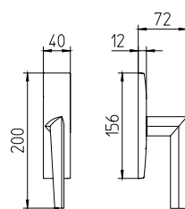
1082/M cremonese window lever handle
