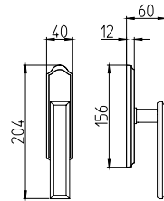
1742/M cremonese window lever handle
