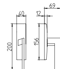
1372/M cremonese window lever handle
