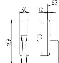
1172/M cremonese window lever handle
