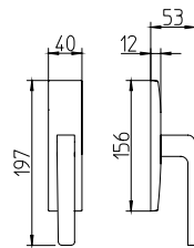
1682/M cremonese window lever handle
